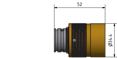
TrustLink Metal Shell CCP
