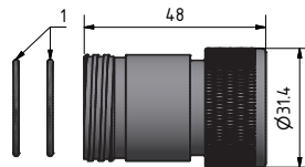
TrustLink Metal Shell Male Pressure Cap
