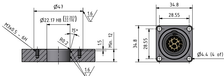
Mounting hole for FCR SB
