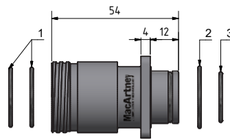
TrustLink Metal Shell FCR SB
