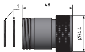
TrustLink Metal Shell Male Pressure Cap
